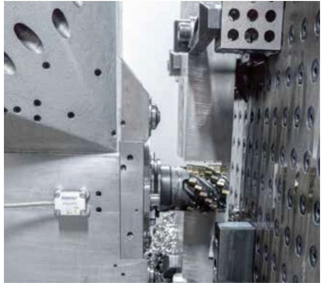
3 As part of testing to produce slots using a five-bladed 80-mm sprocket cutter, there were machining processes with virtually no measurable vibrations (© Burkhardt+Weber)
